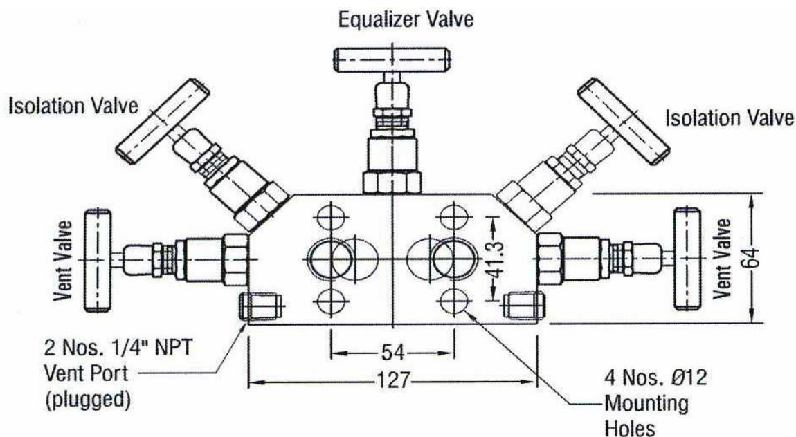
MODEL: Coplanar Direct Mount 5-Valve Manifold - Side Venting
